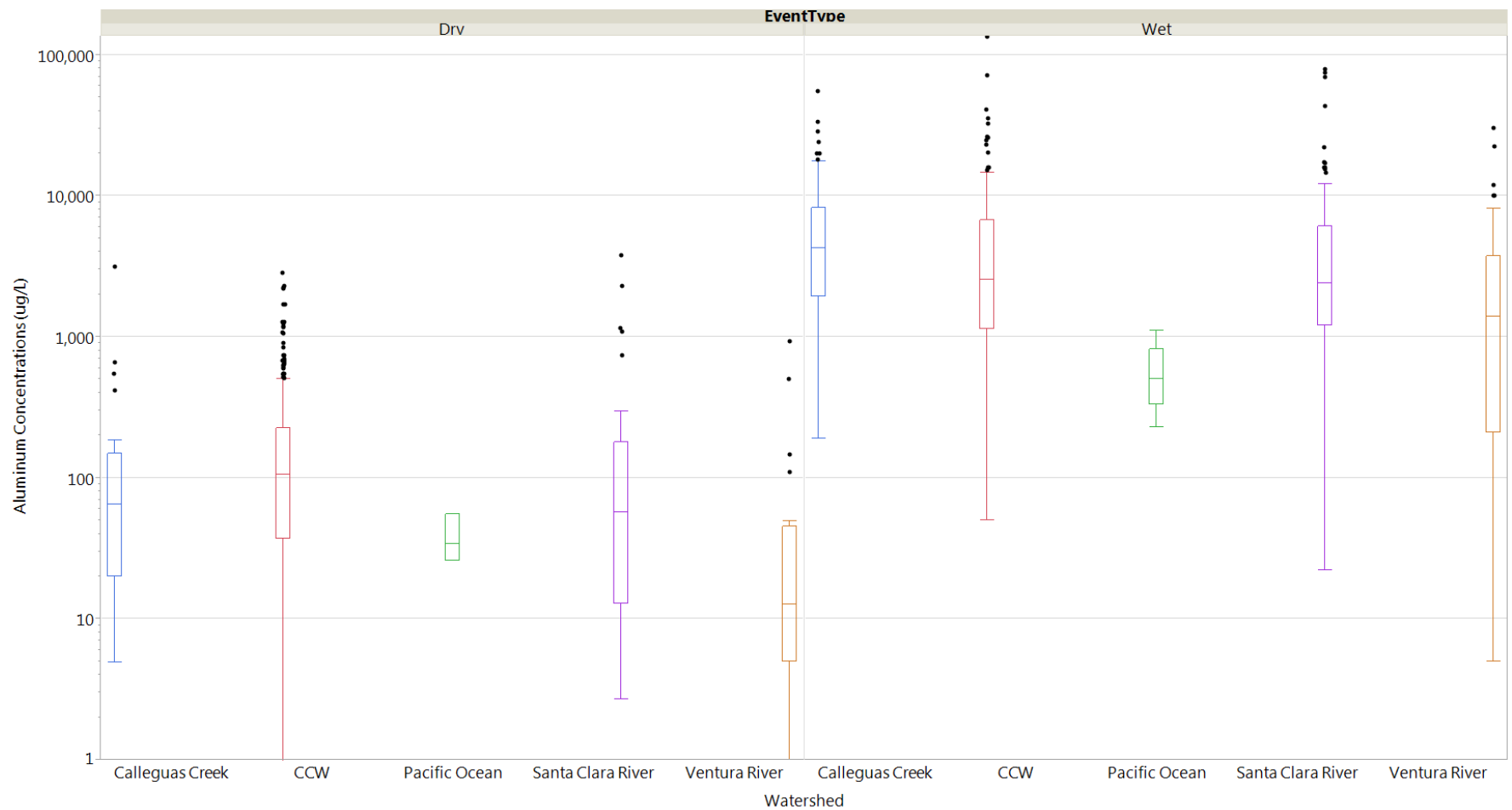
Figure 3: Comparison by Watershed of Total Aluminum Concentrations Measured during Dry and Wet Weather Monitoring Events. (All plotted data collected by VCSQMP except for Calleguas Creek Watershed "CCW" data collected by the CCWTMP)
