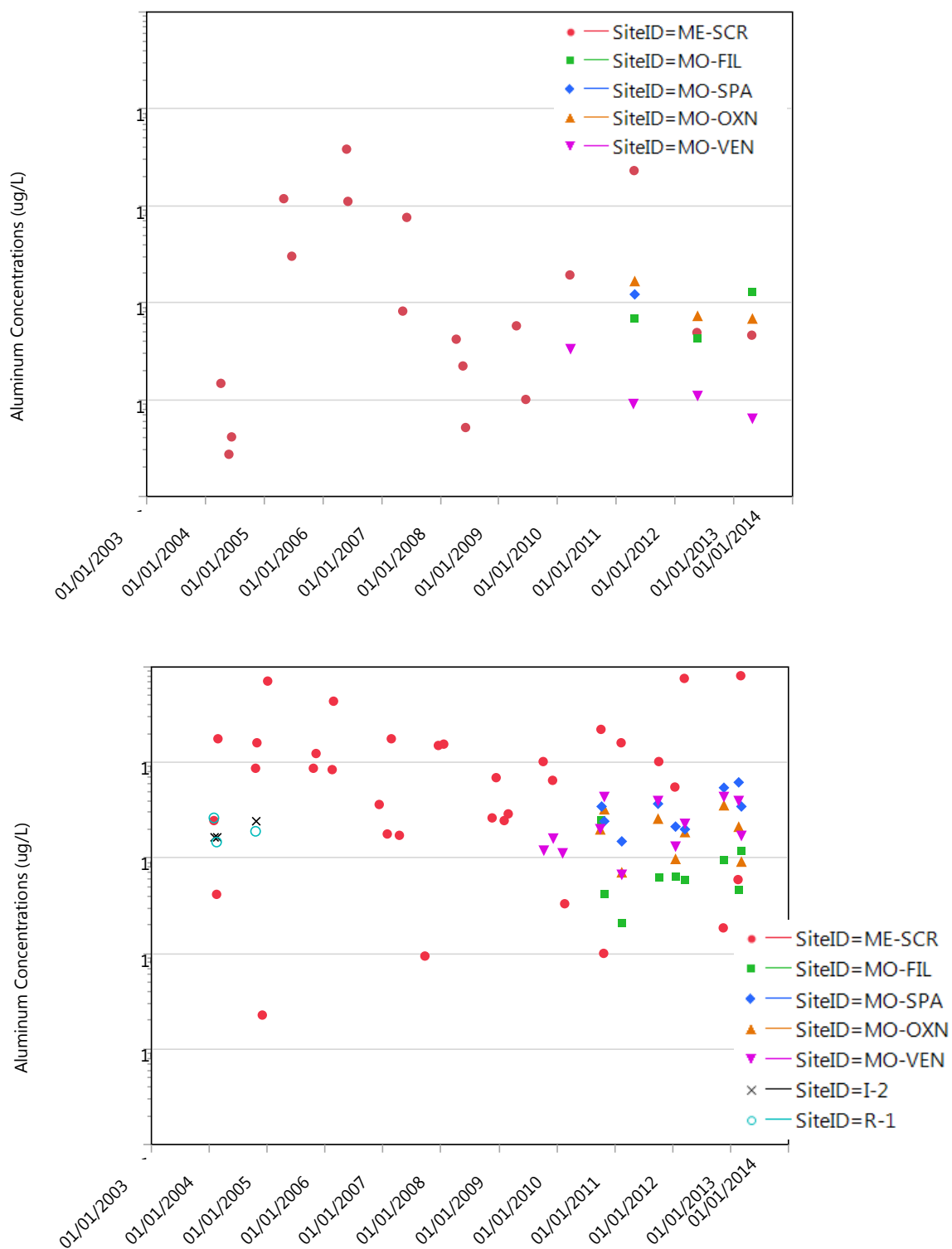
Figure 5: Santa Clara River Watershed Total Aluminum Concentrations Measured by VCSQMP [Dry Weather (top) and Wet Weather (bottom)].
