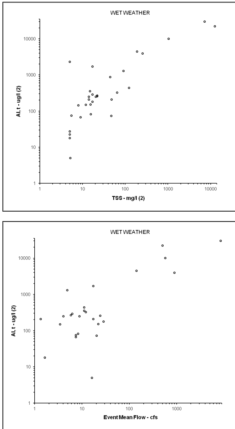
Figure 14: Scatter Plots of Aluminum Vs Event Mean Flow and Aluminum Vs TSS for Wet Weather Data Collected at the Ventura River Mass Emission Site, ME-VR(2).
