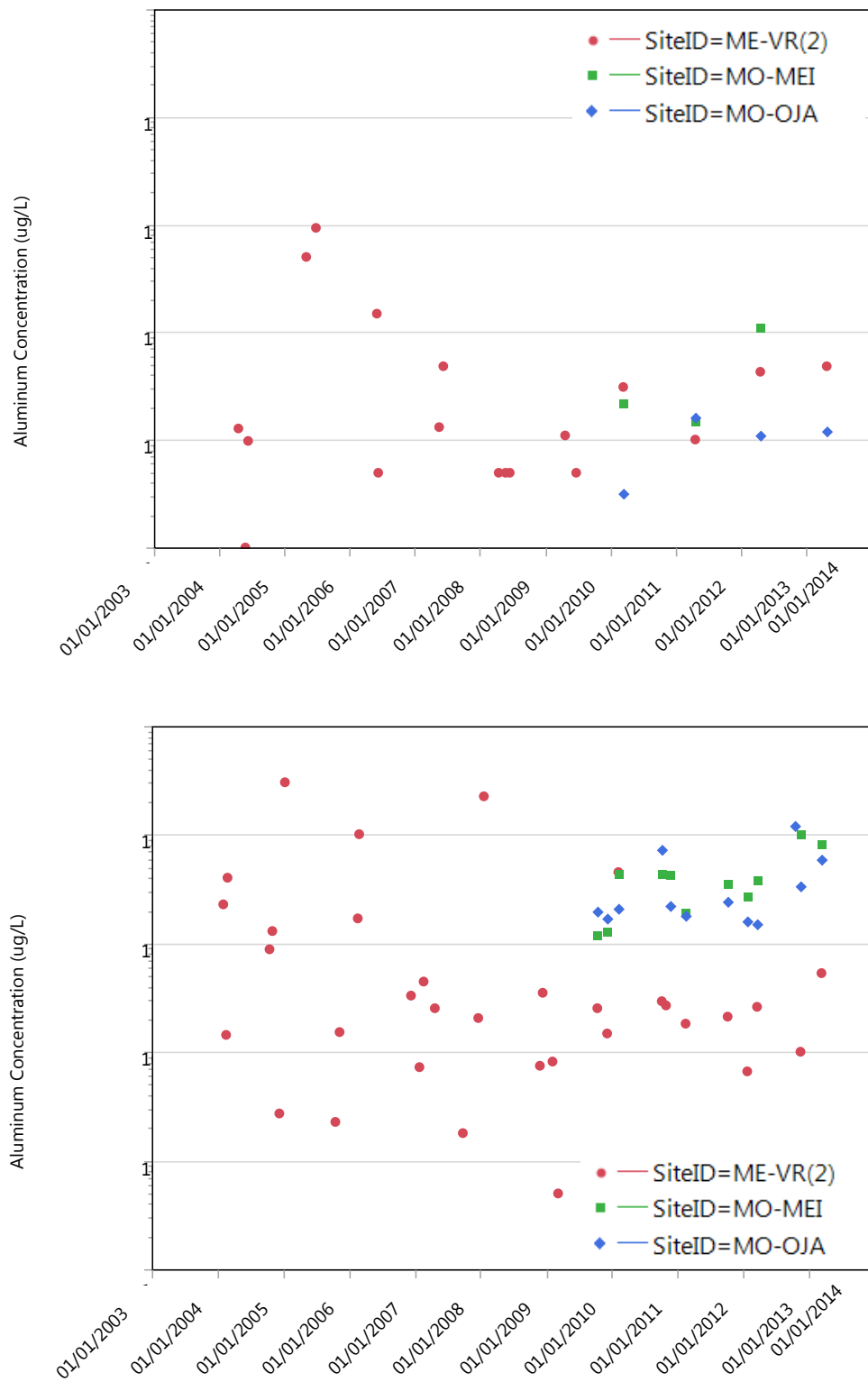
Figure 4: Ventura River Watershed Total Aluminum Concentrations Measured by VCSQMP [Dry Weather (top) and Wet Weather (bottom)].
