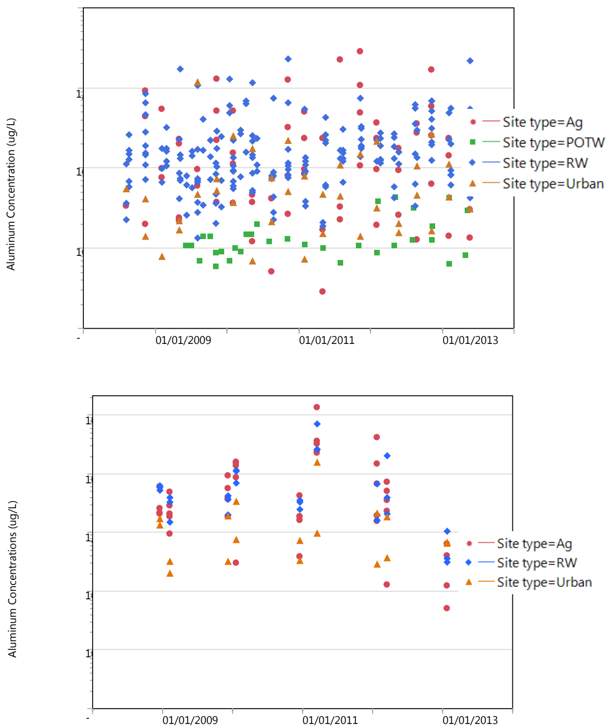
Figure 7: Calleguas Creek Total Aluminum Concentrations Measured by CCWTMP [Dry Weather (top) and Wet Weather (bottom)].
